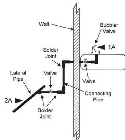
Targeted Locations of Water in Plumbing for Samples 1A & 2A
